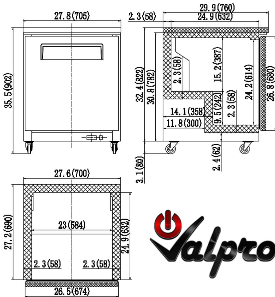
Dimensional Drawing HC-VPUCR27 / HC-VPUCF27
