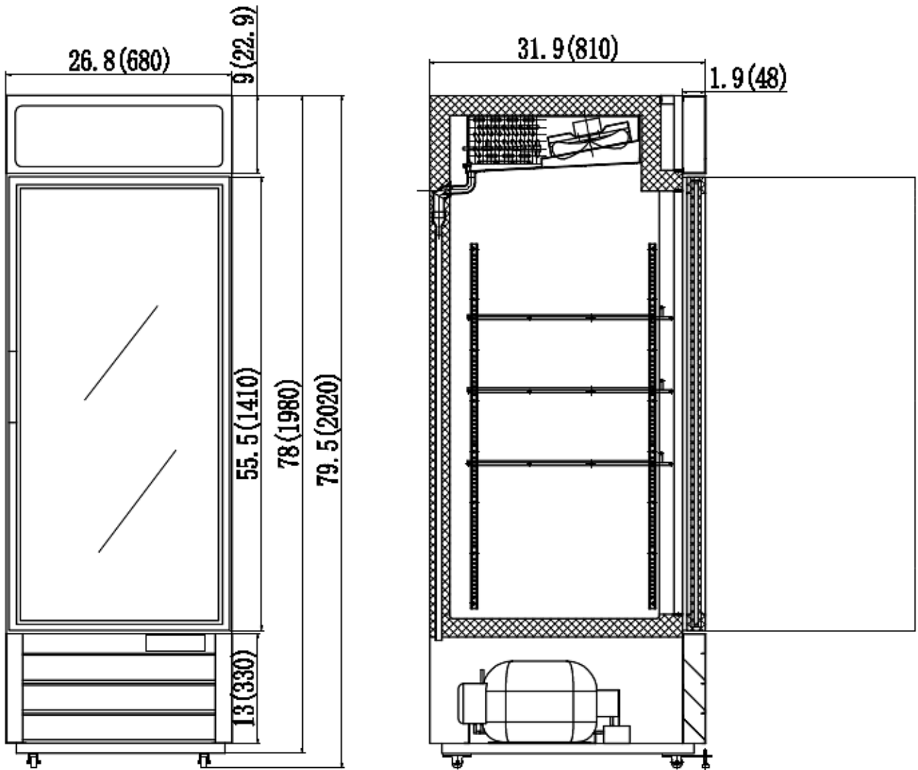
Dimensional Drawing VP1R-23 / VP1R-23
