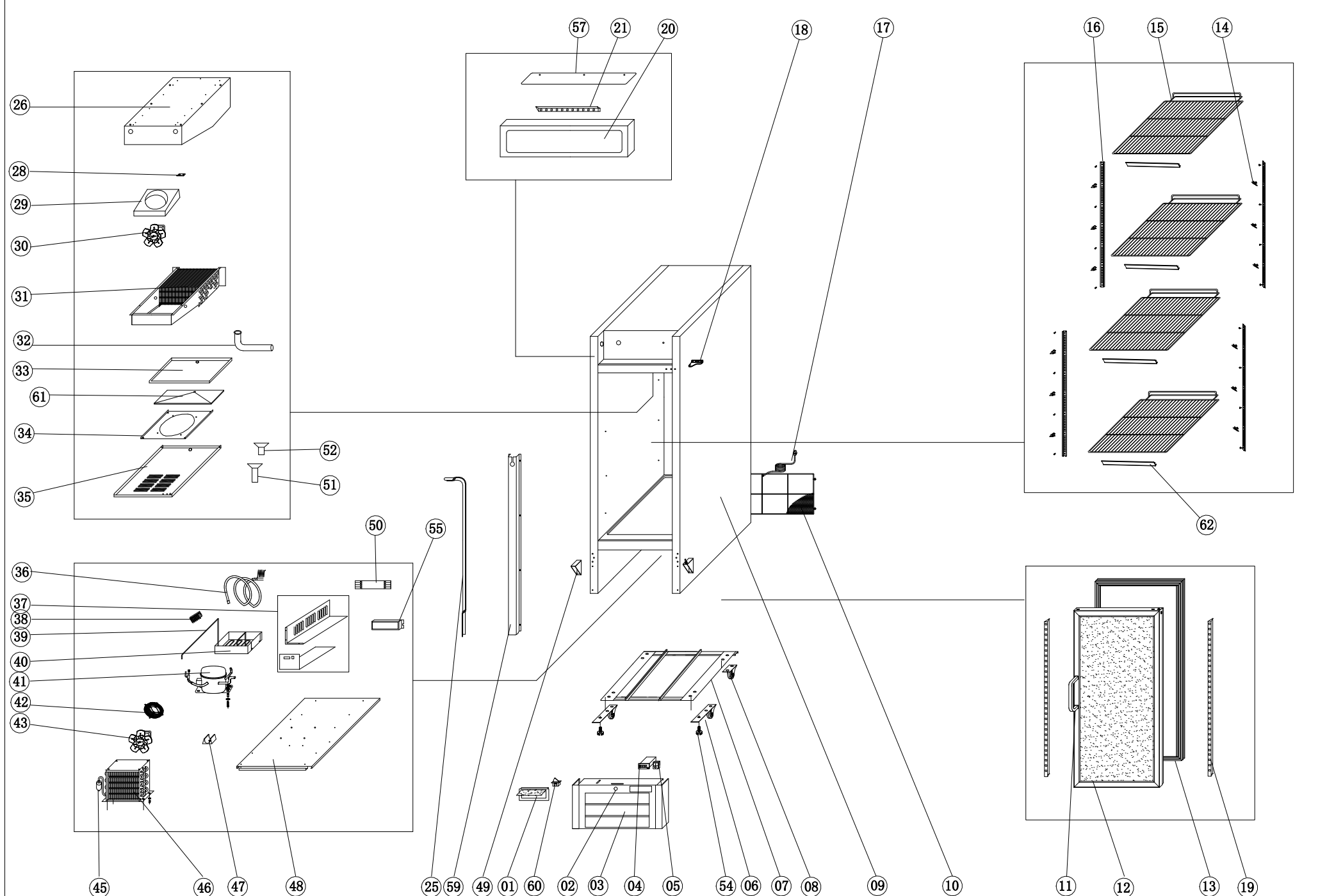
EXPLODE OF: VP1R-23HC
