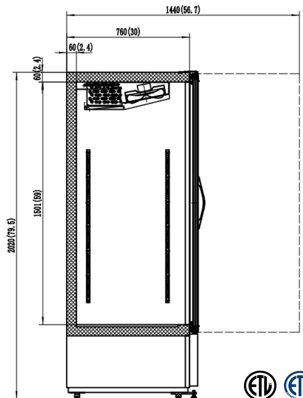
SIDE VIEW
